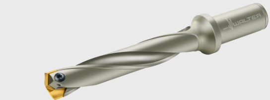
03 Walter Xtra-tec® Point Drill B4015
